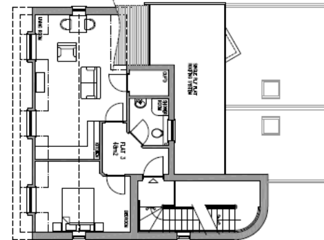
Proposed Second Floor
